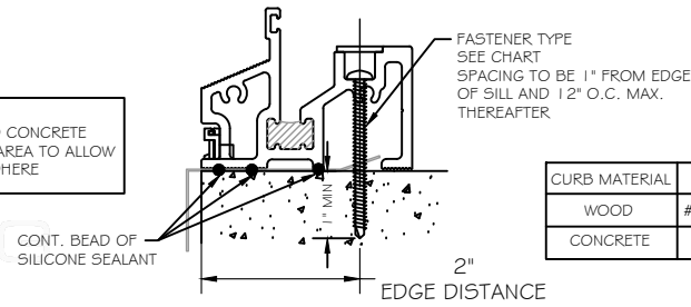
G-G INSWING SILL ANCHORING
