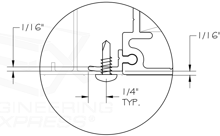
⊗ DETAIL
