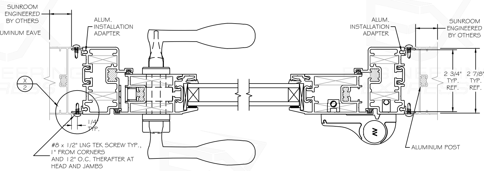
(C-C) HORIZONTAL SECTION
