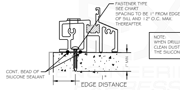
D-D OUTSWING SILL ANCHORING
